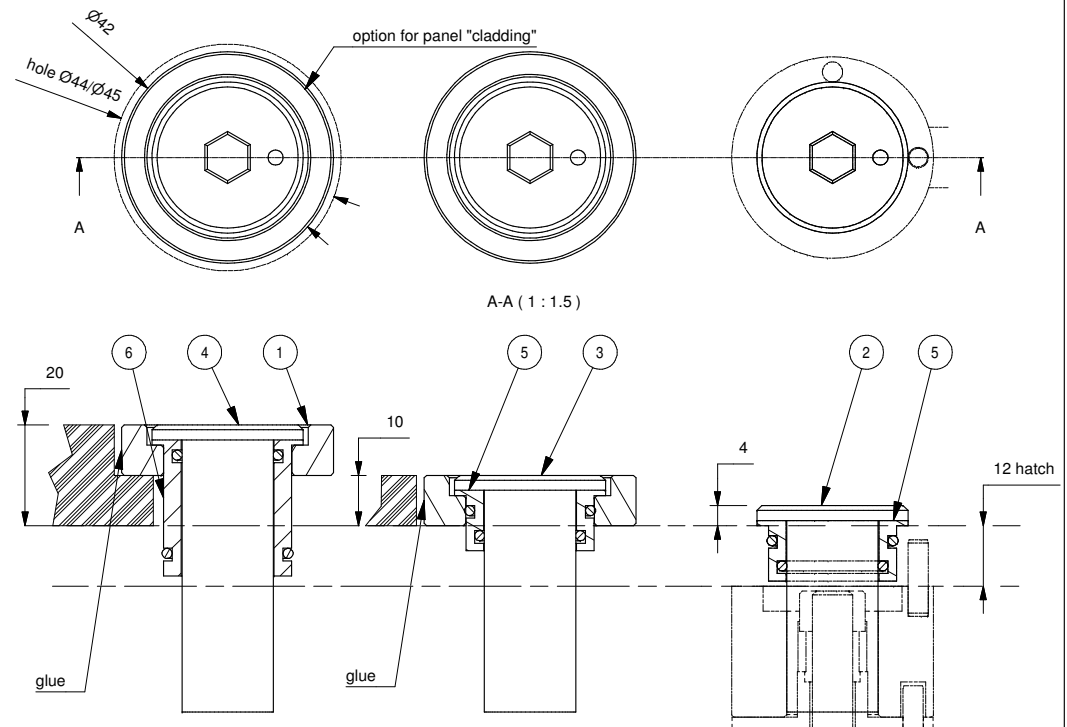
Hex (standard) key
