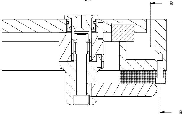
Extruded type frame
