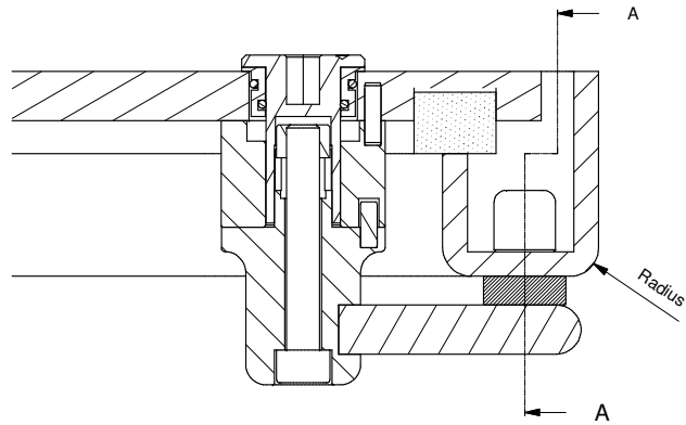
Sheet metal type frame
