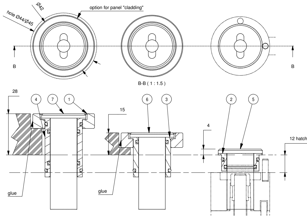
Lifting key
