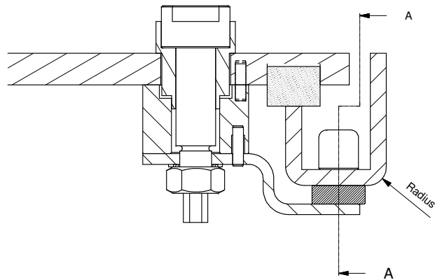
Sheet Metal Frame
